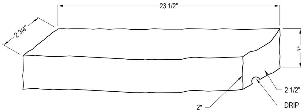
PERSPECTIVE - WATER TABLE SILL
