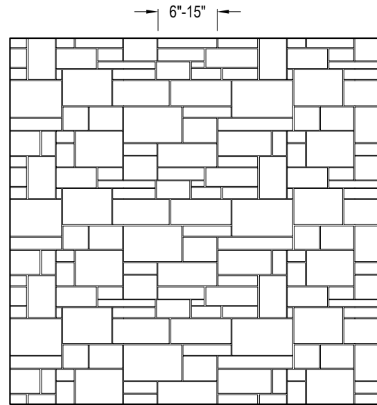
FRONT ELEVATION - DRESSED ASHLAR
