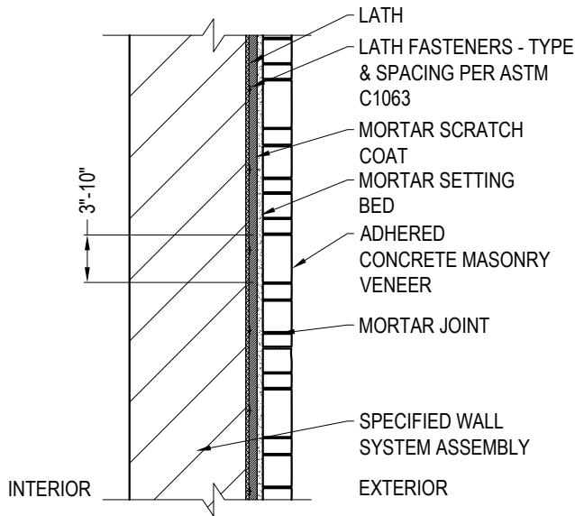
TYPICAL SECTION
