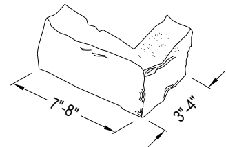
CORNER DETAIL
